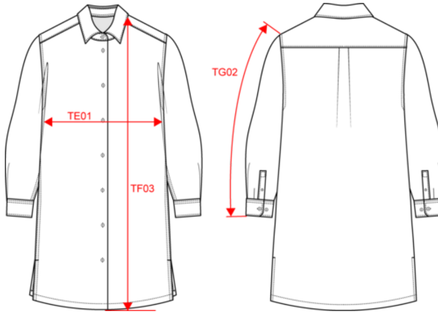
Dimensions (cm)
